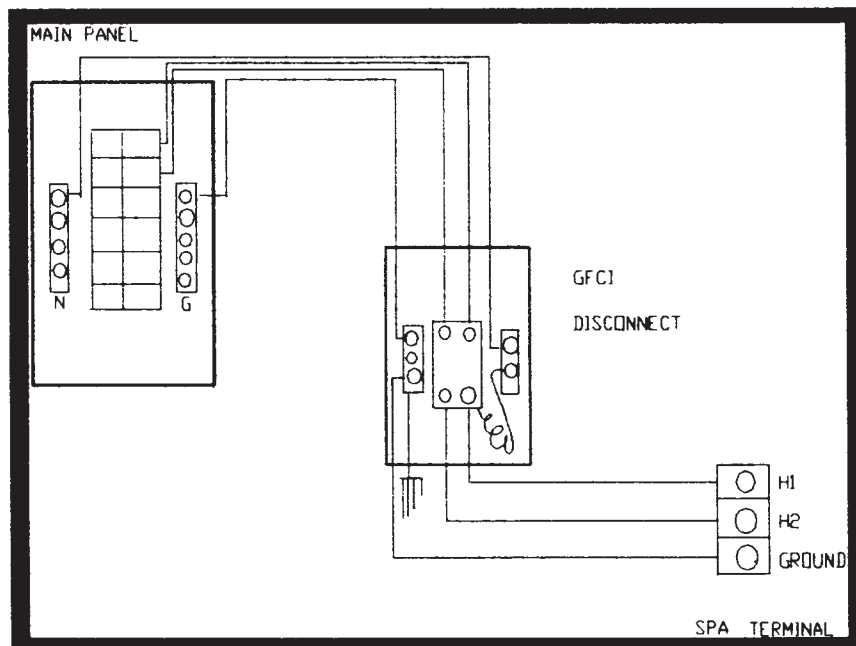
SEPARATE NEUTRAL & SOLID GROUND
